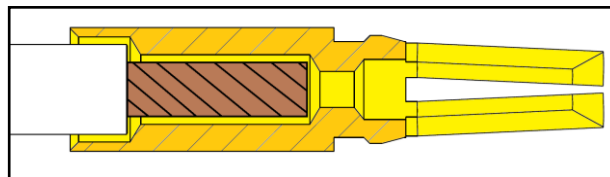
Figure C - All strands in inner crimp bore
