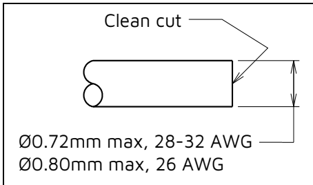
Figure A - Clean cut end
