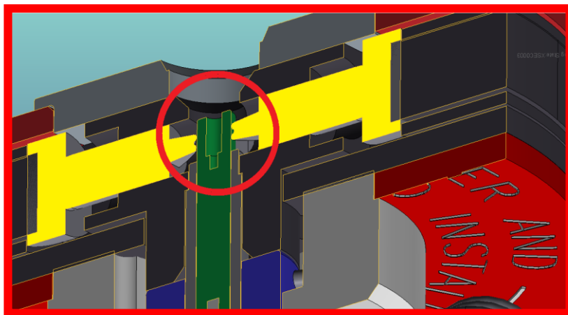
Figure H – Damage risk if the positioner is not fully back to default position
