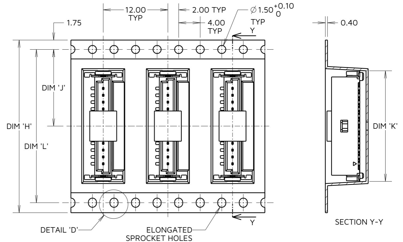
TAPE DETAILS FOR 8 TO 12 CONTACT CONNECTORS
