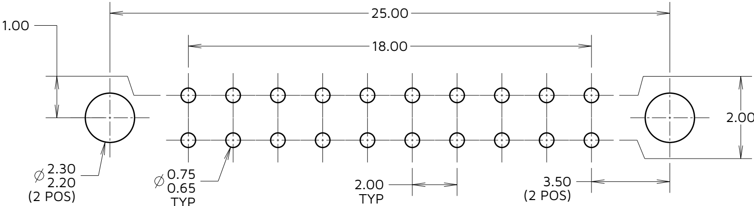
RECOMMENDED PCB LAYOUT TOLERANCE \pm 0.05\text{mm} (UNLESS OTHERWISE STATED)
