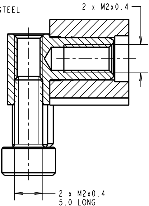
SECTION Z-Z
