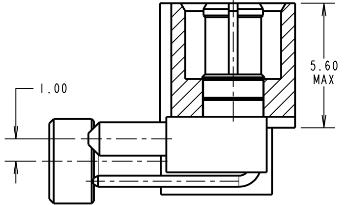
SECTION Y-Y
