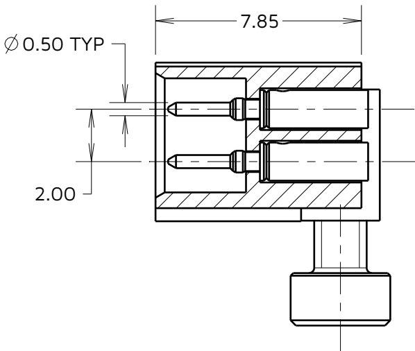
SECTION X-X
